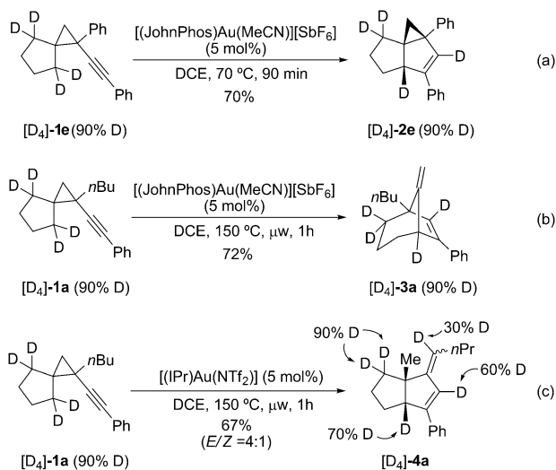
Scheme 6. Deuterium-labeling experiments.
