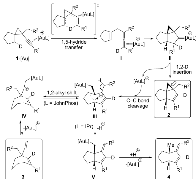
Scheme 8. Proposed mechanism.
